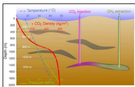
Figure 6 : Coal Bed Methane extraction by liquid CO2 sweeping – Source PhD Thesis of S. Nikoosokhan, U. Paris-Est
