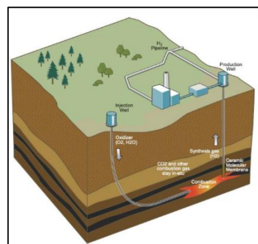
Figure 7 : H 2 production by in situ combustion- Source Bureau of Economic Geology, Texas
